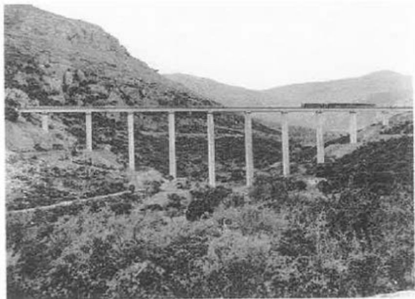
Bridge of Achladolumpos (the first rail bridge in Greece made of cement with pillars of 60m)
